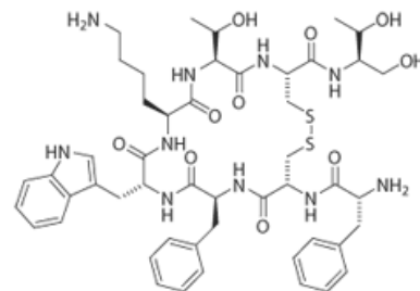
Octreotide acetate
