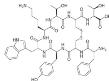
[Tyr 3 ]octreotate acetate
