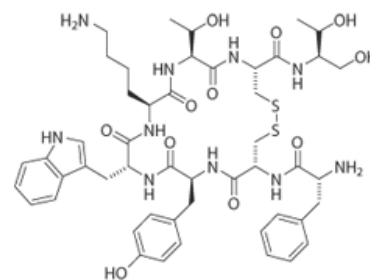
[Tyr 3 ]octreotide acetate
