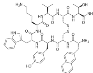
Lanreotide trifluoroacetate
